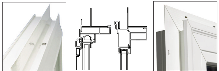
There are more than one style of Integral J-Channel frame profiles.
